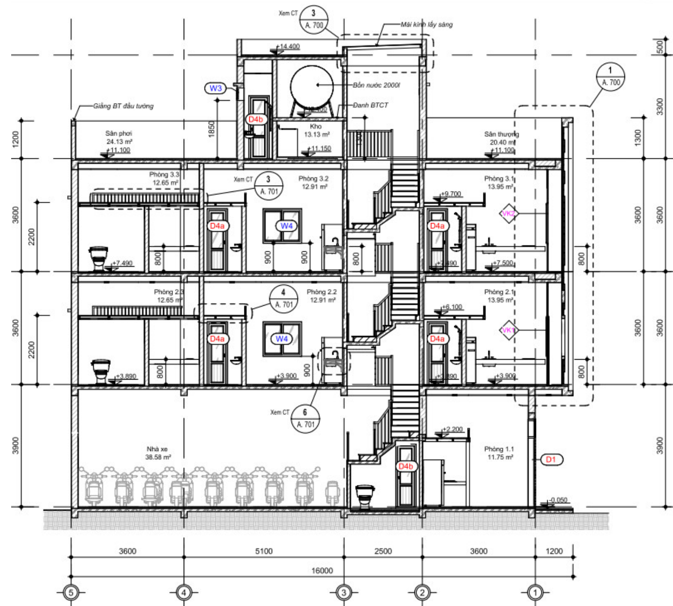
1 MẶT CẮT 1 / BUILDING SECTION 1 1:100
