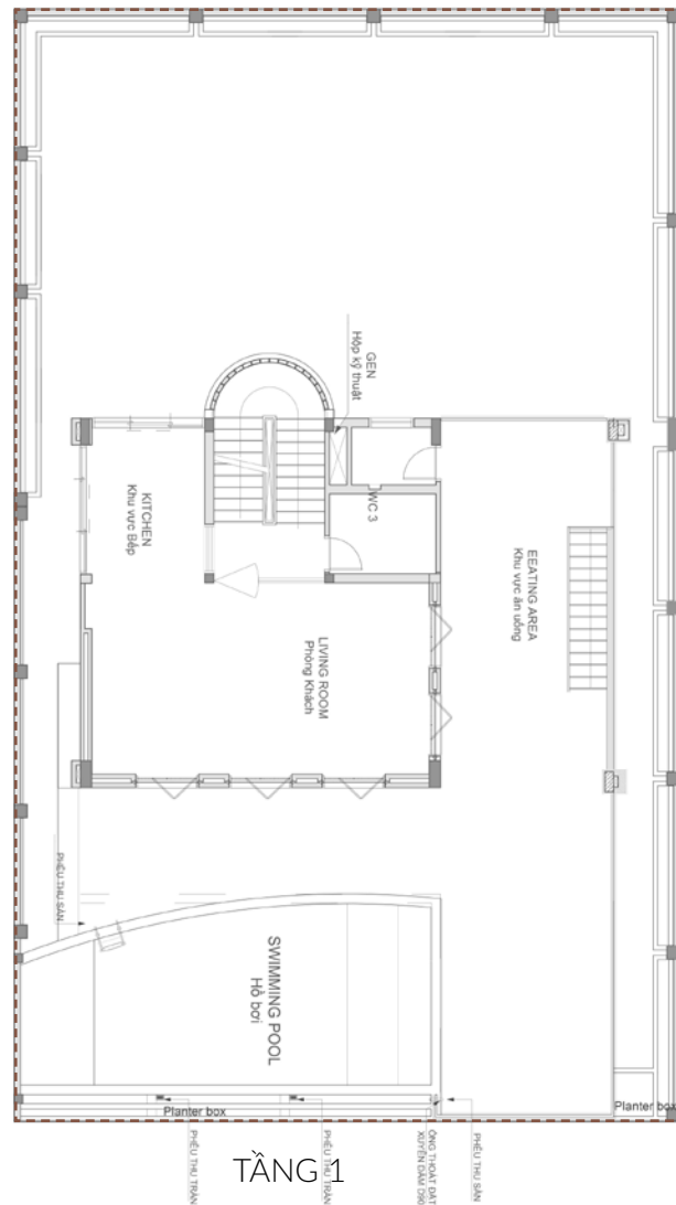
1ST FLOOR
